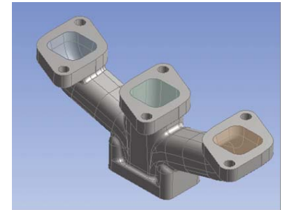
Solid geometry of a manifold
